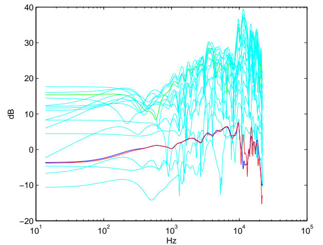
Figure 12: Subdivided interpolated HRTF, complete and measured HRTFs (dark).
